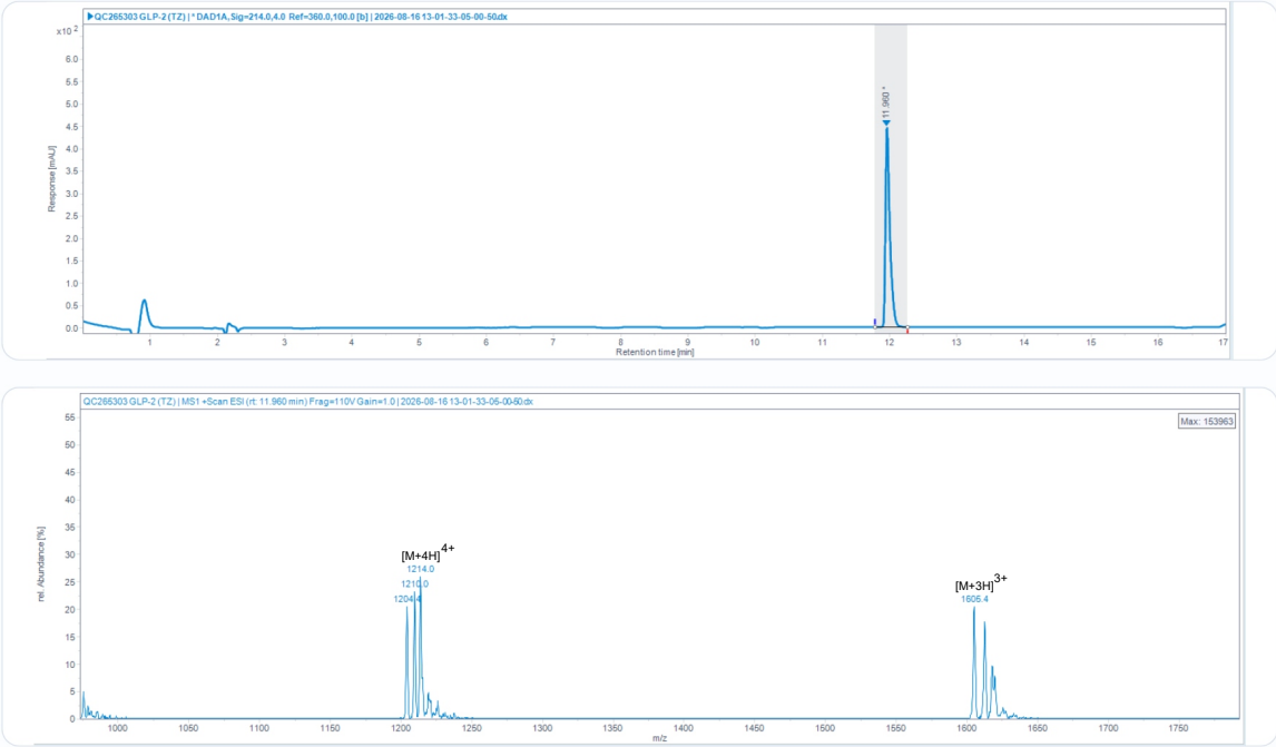
HPLC Chromatogram · Retention Time 11.960 min
